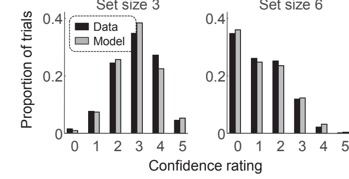
Figure S7. Model fit to data of subject S6. (A) Histogram of estimation errors, split by confidence rating (columns) and set size (rows). (B) Distribution of confidence ratings, split by set size. (C) Circular variance of the estimation error as a function of confidence rating, split by set size. Error bars indicate bootstrapped 95% confidence intervals.
