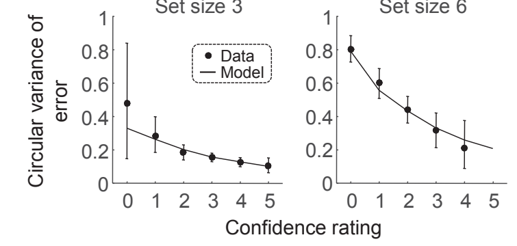
Figure S7. Model fit to data of subject S6. (A) Histogram of estimation errors, split by confidence rating (columns) and set size (rows). (B) Distribution of confidence ratings, split by set size. (C) Circular variance of the estimation error as a function of confidence rating, split by set size. Error bars indicate bootstrapped 95% confidence intervals.
