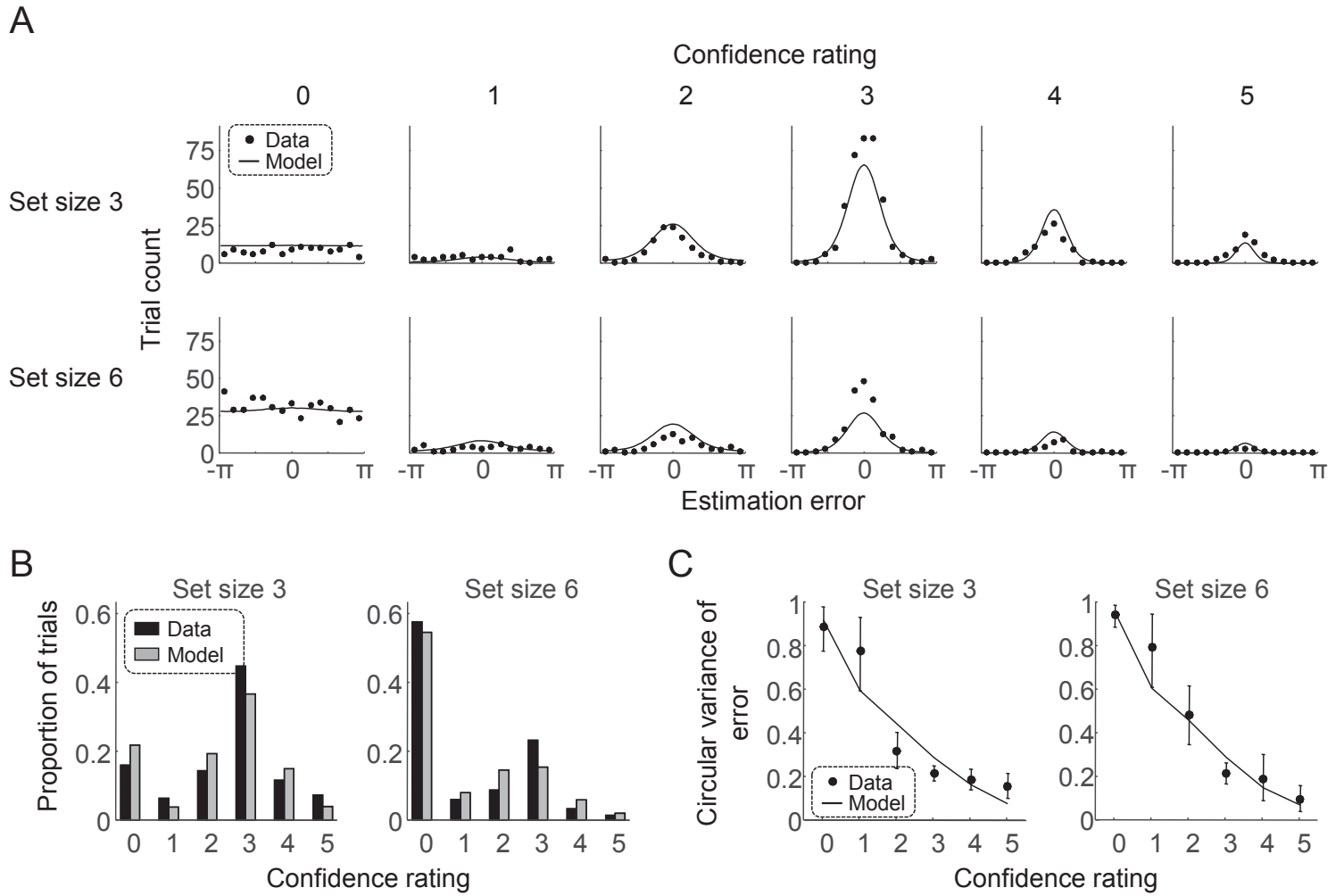
Figure S3. Model fit to data of subject S2. (A) Histogram of estimation errors, split by confidence rating (columns) and set size (rows). (B) Distribution of confidence ratings, split by set size. (C) Circular variance of the estimation error as a function of confidence rating, split by set size. Error bars indicate bootstrapped 95% confidence intervals.
